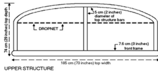
UPPER STRUCTURE
