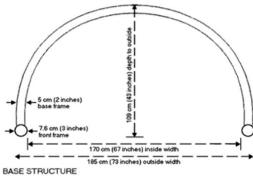
BASE STRUCTURE
