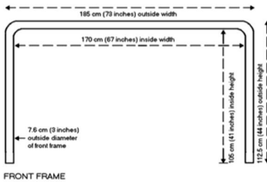
FRONT FRAME
